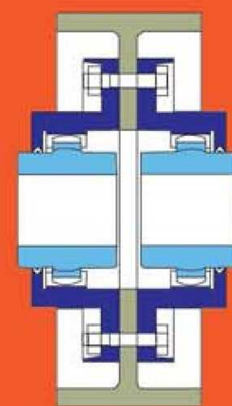
BRAKE DRUM COUPLING
